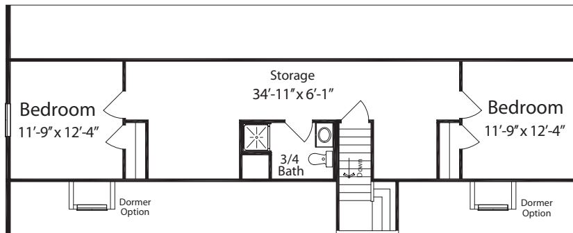
Suggested Second Floor (All work performed on-site by others)
