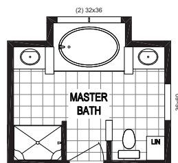
DELUXE MASTER BATH OPTION w/ 48" SHOWER & DECK TUB
