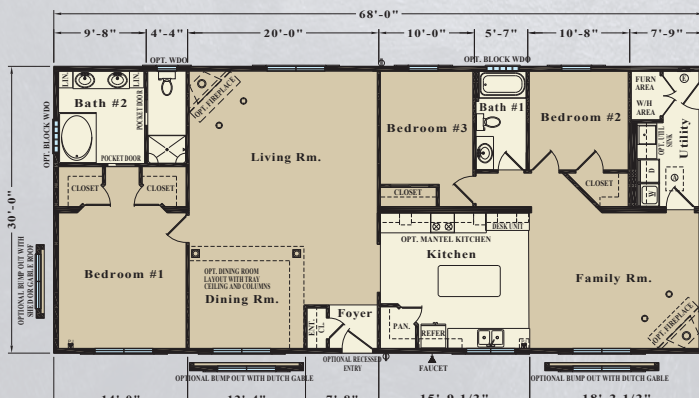
MODEL JR23B - 2,040 S.F.
